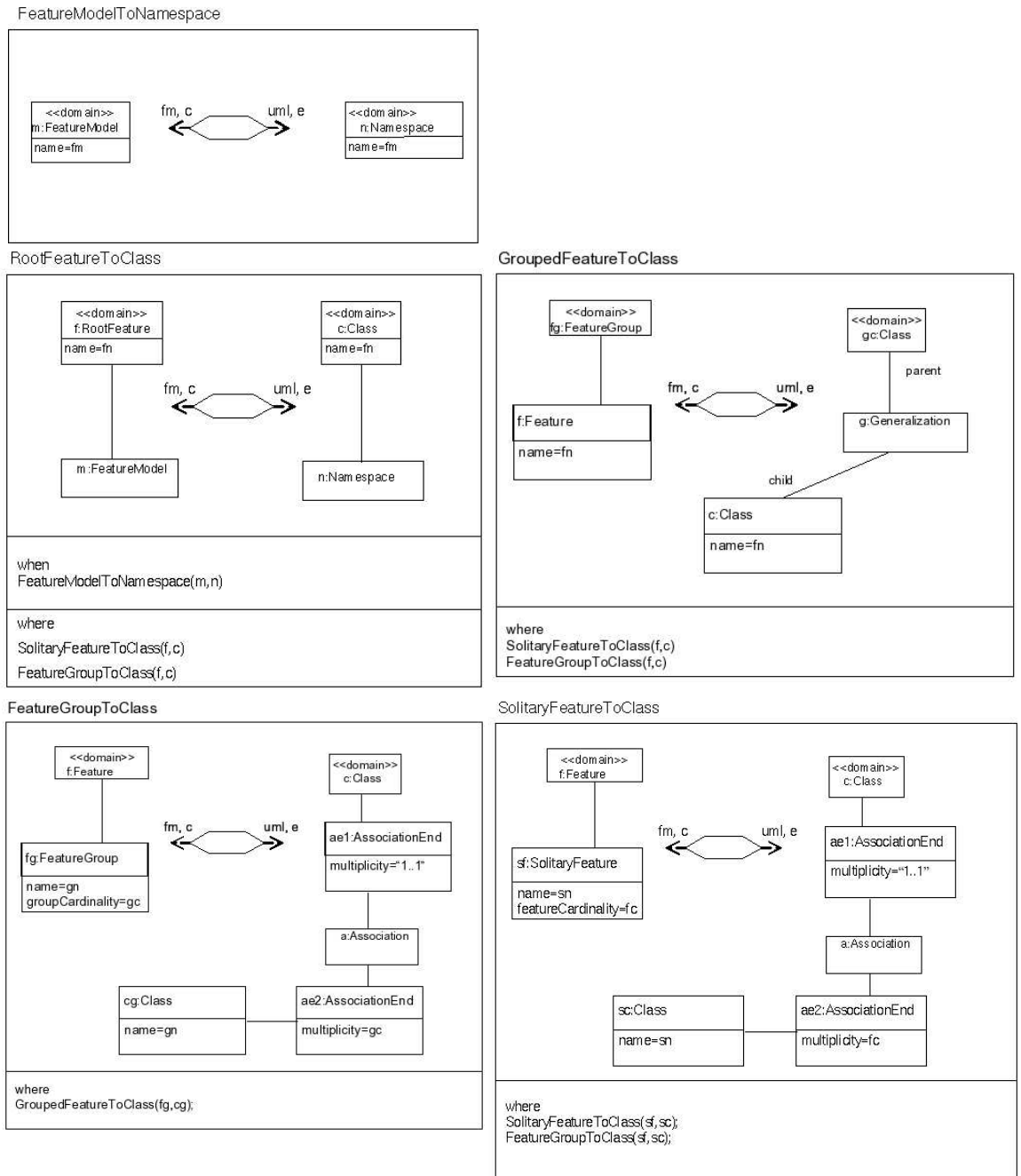
Fig. 5. Transformation definition of a Feature model into a UML metamodel
