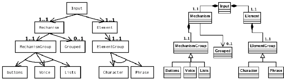
Fig. 2. Feature model in the domain of communication for handicapped people and a simple solution using composition, association, and specialization
